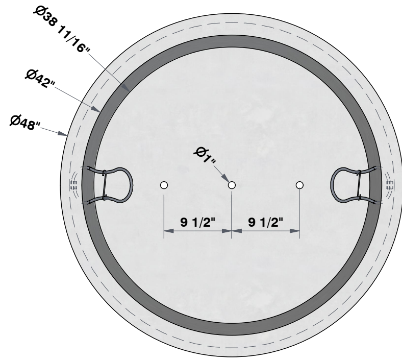
TOP VIEW 7/8"=1'
