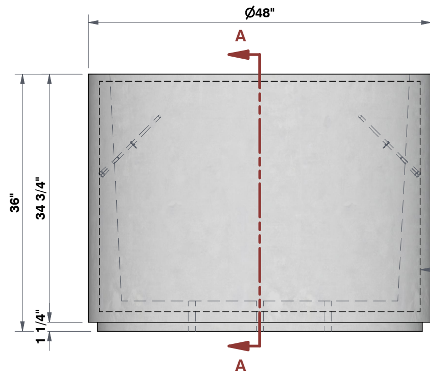
FRONT VIEW 7/8"=1'
