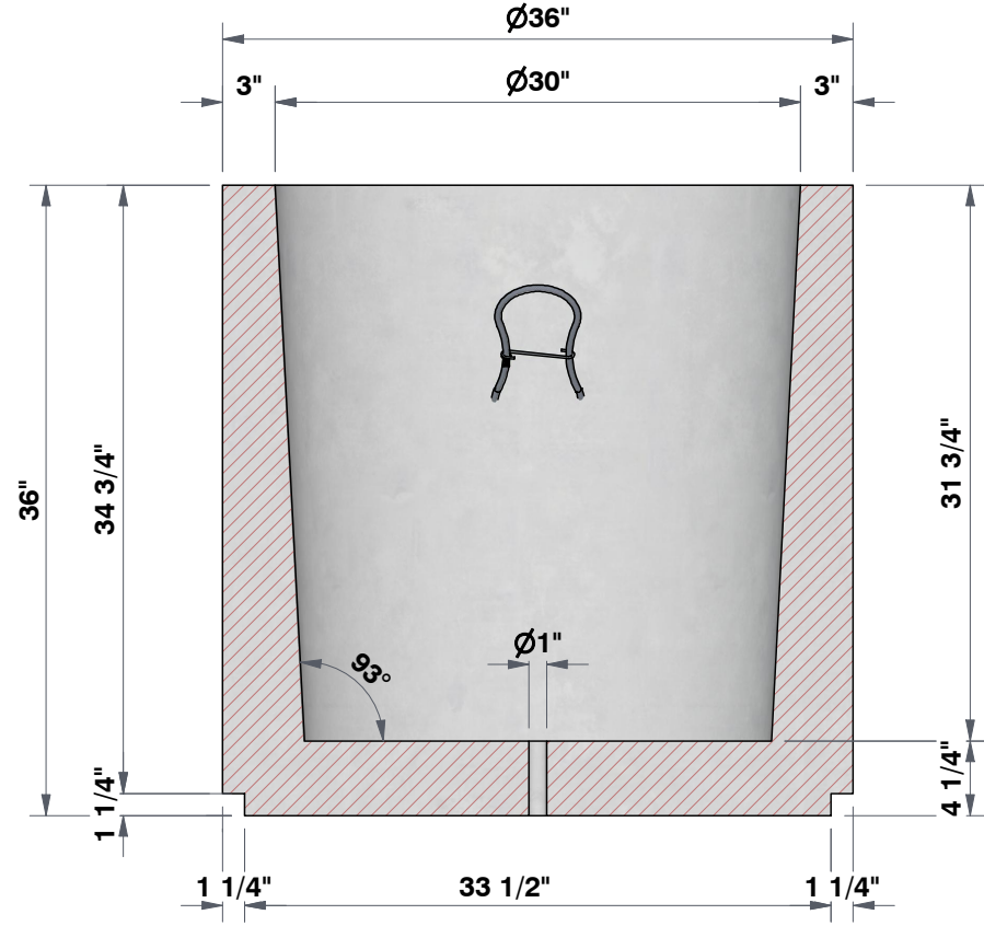
SECTION A-A 1"=1'
