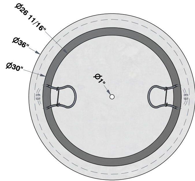
TOP VIEW 1"=1'
