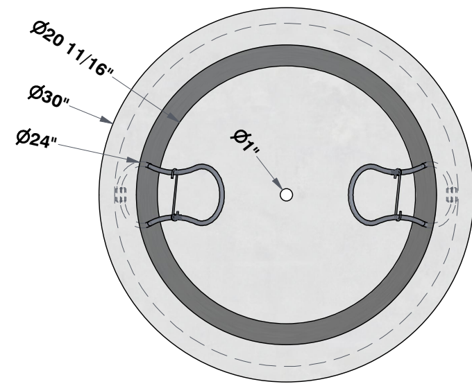
TOP VIEW 1 1/8"=1'
