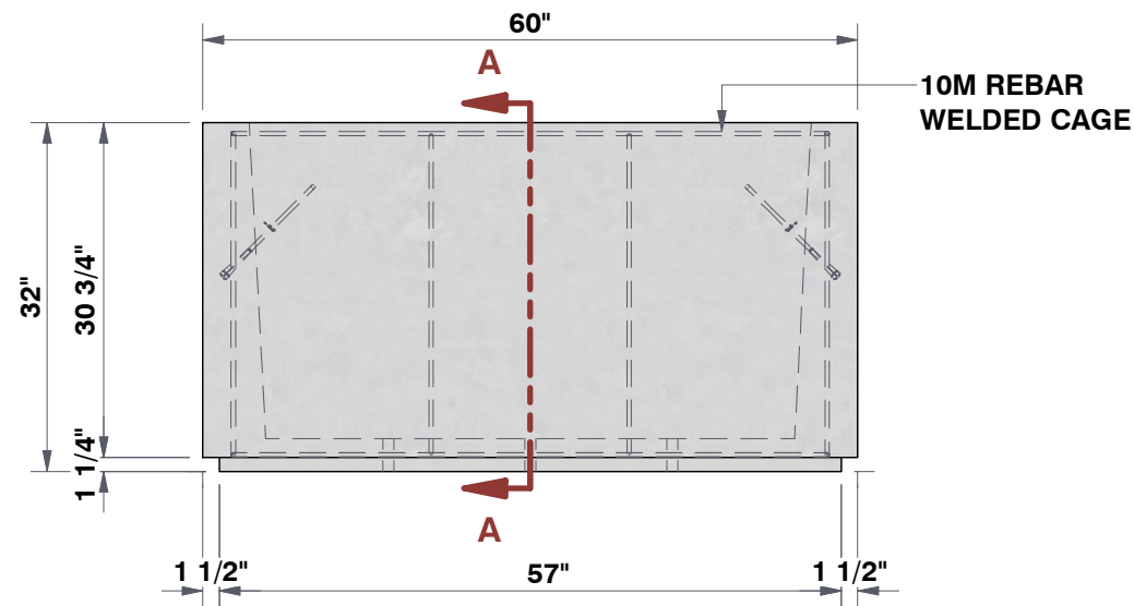
FRONT VIEW 5/8"=1'
