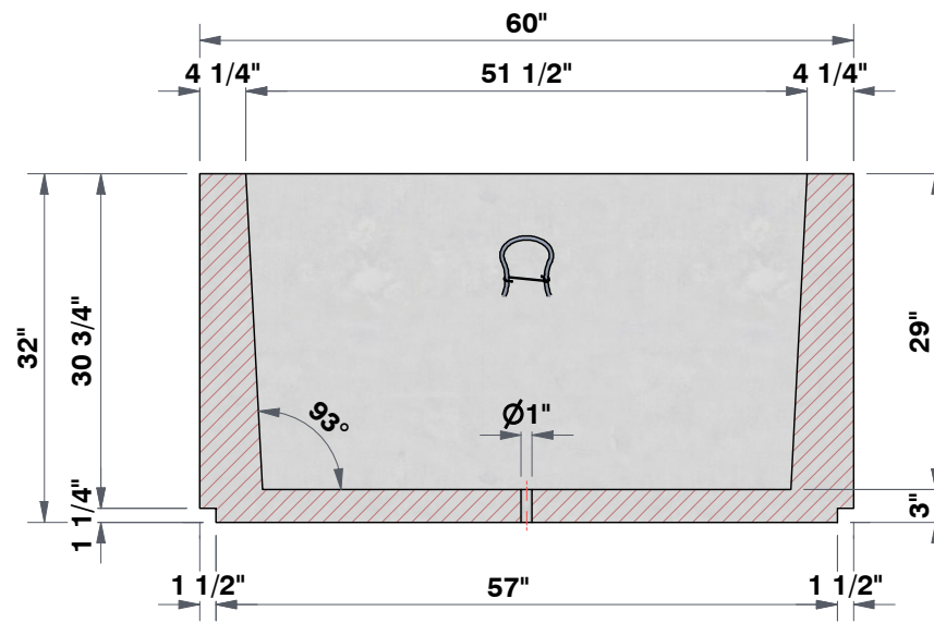
SECTION A-A 5/8"=1'
