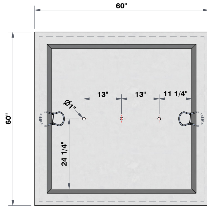
TOP VIEW 5/8"=1'
