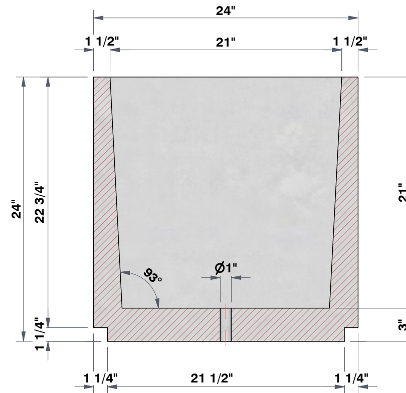
SECTION A-A 1 3/8"=1'
