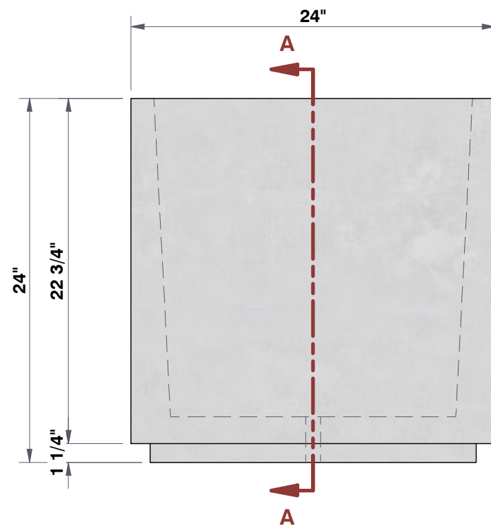
FRONT VIEW 1 3/8"=1'
