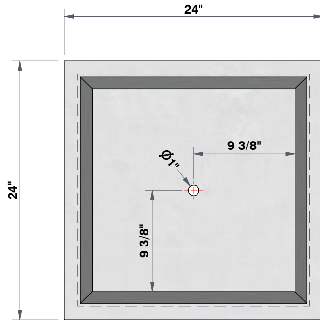
TOP VIEW 1 3/8"=1'
