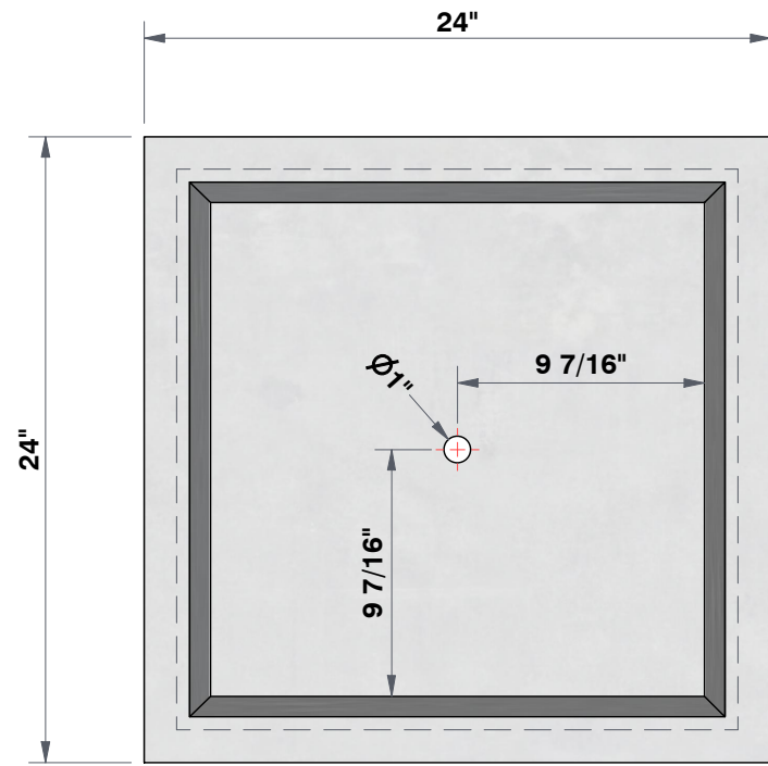
TOP VIEW 1 1/2"=1'
