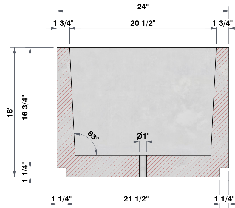
SECTION A-A 1 1/2"=1'
