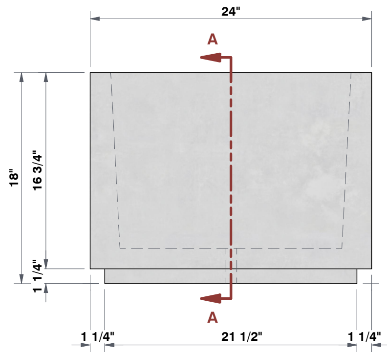
FRONT VIEW 1 1/2"=1'
